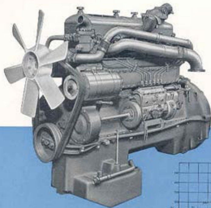
A.E.C. 11-3 liter down-injection oil engine
